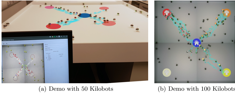
Fig. 6. (a) Image from demo D3 with n = 4 source areas. In the closeup, the computer screen shows the ARK’s virtual environment, on the background the Kilobots move between virtual sources following virtual pheromone trails (the virtual environment has been superimposed to the image). (b) Screenshot from demo D4 . Full videos are available at http://diode.group.shef.ac.uk/FontLlenas2018.html .
