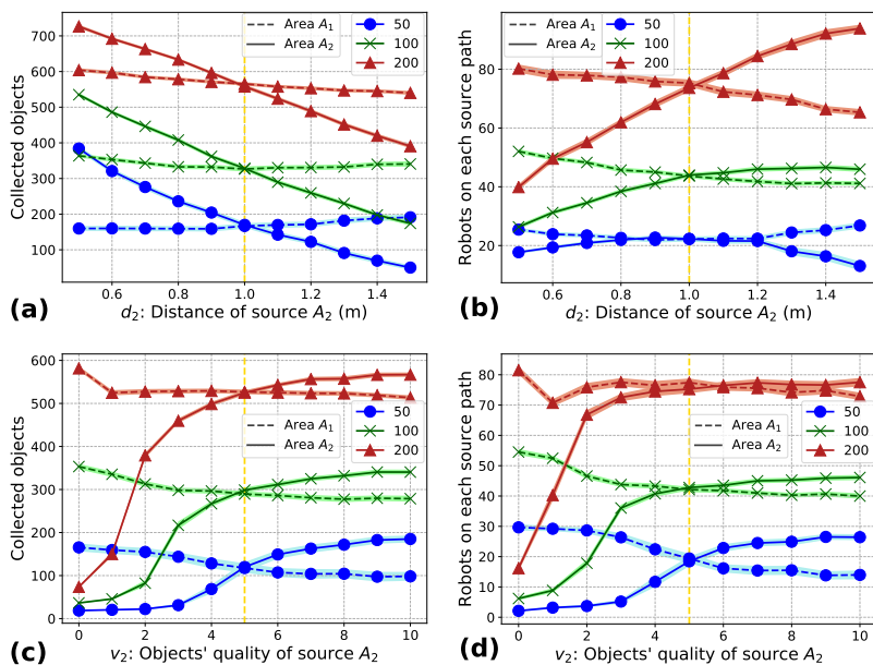
Fig. 3. Results from simulation experiments with S = \{50, 100, 200\} Kilobots and two source areas with (a)-(b) equal quality, varying distance, and (c)-(d) equal distance, varying quality. In (a),(c) we report the number of collected objects after 20 minutes; in both cases, the closest, or better quality, source area has a larger number of collected items. In (b),(d) we report the number of robots on each source path after 20 minutes. Small swarms allocate resources differently than larger swarms. Lines are mean of 100 simulations and the lighter colour fill is the 95% confidence interval.
